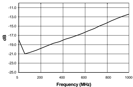
Directivity
